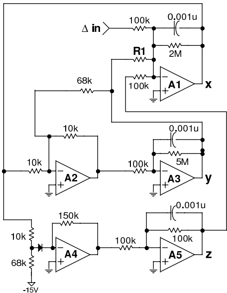
FIG. 1: The experimental setup. Rössler-like circuit used to generate data. For the first (the second) circuit, the resistor R1 was 221\text{ k}\Omega ( R1 = 178\text{ k}\Omega ).
