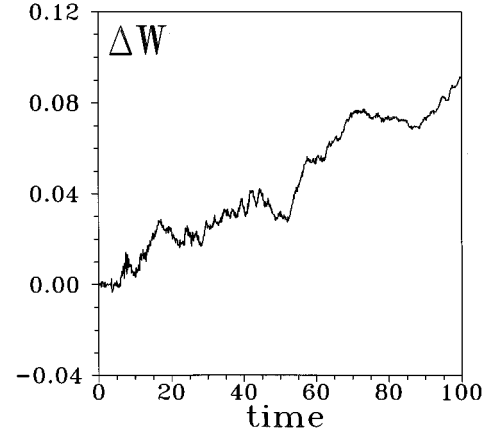
FIG. 3. Differences \Delta W (see text) between quantum and classical integrated Wigner functions extracted from the solution of Eq. (4) with \epsilon=0.7, \hbar=1/200\pi , and 0, respectively. Same boundary and initial conditions as in Fig. 2.
