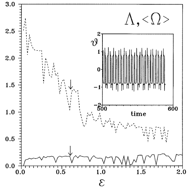
FIG. 1. Maximum Liapunov exponent \Lambda (solid line) and averaged twisting frequency \langle \Omega \rangle (dashed line) as functions of the forcing amplitude \epsilon for the driven double-well system. \Lambda and \langle \Omega \rangle have been evaluated for the classical system [Eq. (5)] with \alpha=1 , \beta=2 , m=1 , \omega=2.5 . Arrows indicate a possible choice for which \langle \Omega \rangle \gg \Lambda . Inset: Temporal evolution of the angle \theta formed by the eigenvector corresponding to the local maximum expansion direction with respect to the x axis. \theta has been calculated for \epsilon=0.7 and the above values of the other parameters.
