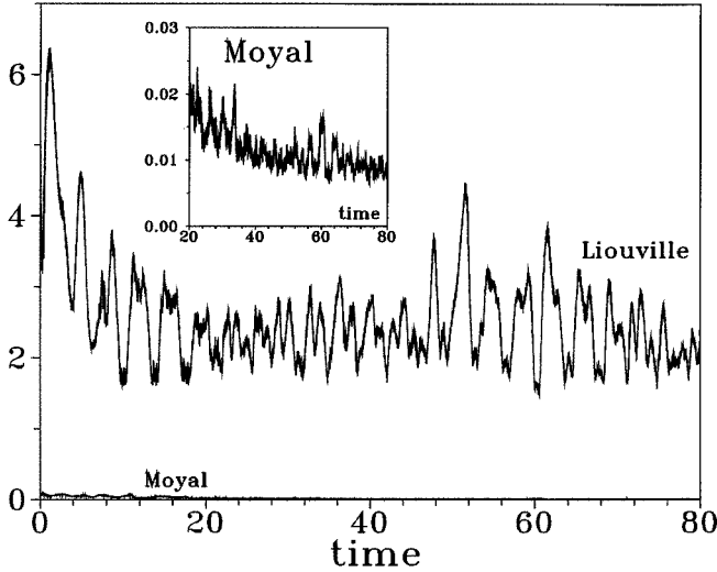
FIG. 2. Plot of the maxima of the Liouville and Moyal terms in the course of time for \epsilon=0.7, \hbar=1/200\pi and other parameters as in Fig. 1. A Gaussian wave packet centered in x=0.3 and p=0.1 whose Wigner function is W(q,p) = (1/\pi\hbar)e^{-(x-x_0)^2/\delta^2 - [(p-p_0)^2\delta^2/\hbar^2]} ( \delta=0.1 ) has been chosen as an initial condition. Boundary conditions as discussed in the text. Inset: vertically magnified plot of Moyal contributions. Notice that the windows confining the Moyal term remains limited, even for t > \tau_1 \approx (1/\Lambda)\ln(S/\hbar) \sim 50 sec.
