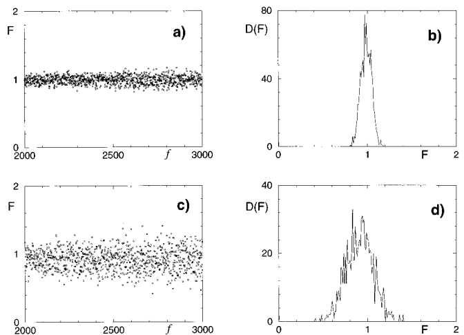
FIG. 8. (From Ref. 30.) Accuracy in the Fourier space reconstruction for MG plus coloured noise (all plots limited to the frequency range covered by the noise). (a) and (c) report the dimensionless quantity F (see text for definition) vs the frequency channel number f for \theta=0.1 and \theta=0.07 respectively. (b) and (d) show the corresponding histograms D(F) vs F . Same parameters as in Fig. 5.
