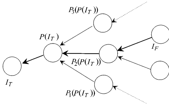
FIG. 15. (From Ref. 57.) Procedure for the construction of the goal dynamics. Each bubble represents the neighborhood of a point in the phase space. I_T : target; P(I_T) : unique preimage of the target; P_j(P(I_T)), j=1,2,3 : multiple preimages of P(I_T) ; I_F : most frequently visited parallelogram. The selected path is shown as a thick line.
