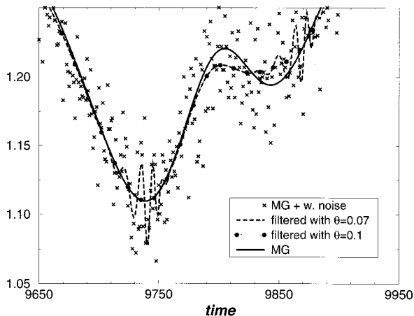
FIG. 6. (From Ref. 30.) Time domain reconstruction of the signal for MG plus white noise. Symbols and lines in the legend. Same parameters as in Fig. 5. Time is in sampling units, the y-axis is labeled in arbitrary units.
