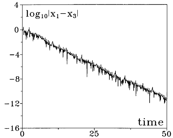
FIG. 13. (From Ref. 55.) Temporal evolution of the quantity \log_{10}|x_1 - x_3| measuring the degree of synchronization between Alice and Bob. \sigma = 0.011 , K = 0.1 .
