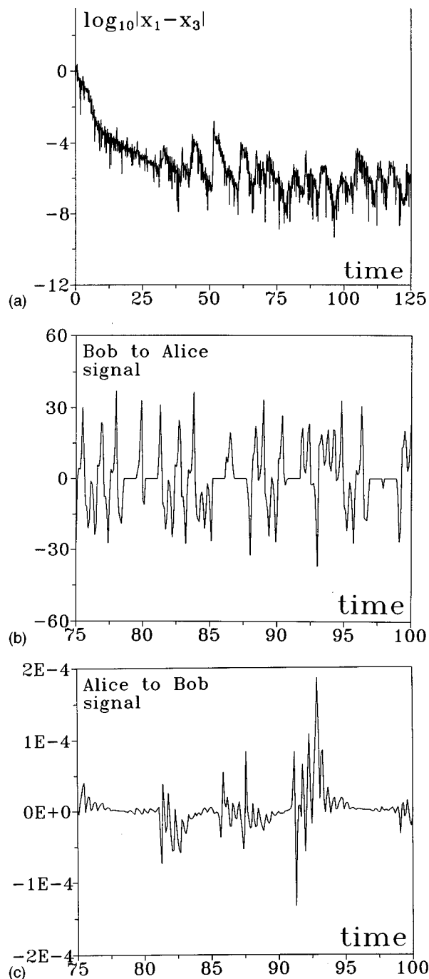
FIG. 14. (From Ref. 55.) (a) Temporal evolution of \log_{10}|x_1 - x_3| for \theta = 10^{-5} and T_0 = 1 . (b) The signal that Bob sends to Alice is affected by large holes, that prevent any possible reconstruction of the message. (c) The controlling signal is kept within a negligible range with respect to the dynamics. Other parameters as in Fig. 13.
